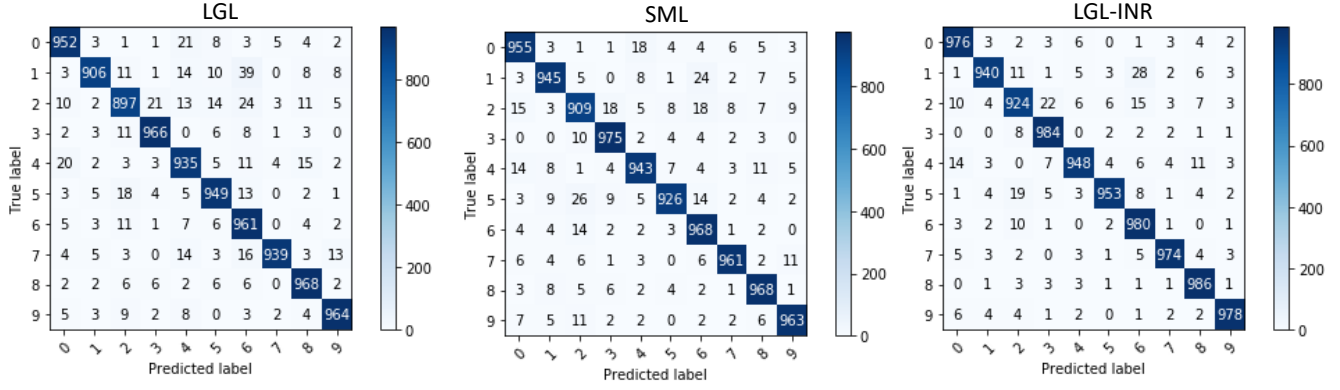
Figure 1: Confusion matrix on MNIST testing data for LGL, SML and LGL-INR. Model: CNN2C. See Table 3 for overall accuracy. Notably, LGL-INR outperforms LGL in all 10 classes and SML in 9 classes except Class 1 (LGL-INR 940 vs. SML 945), in terms of per-class accuracy.
